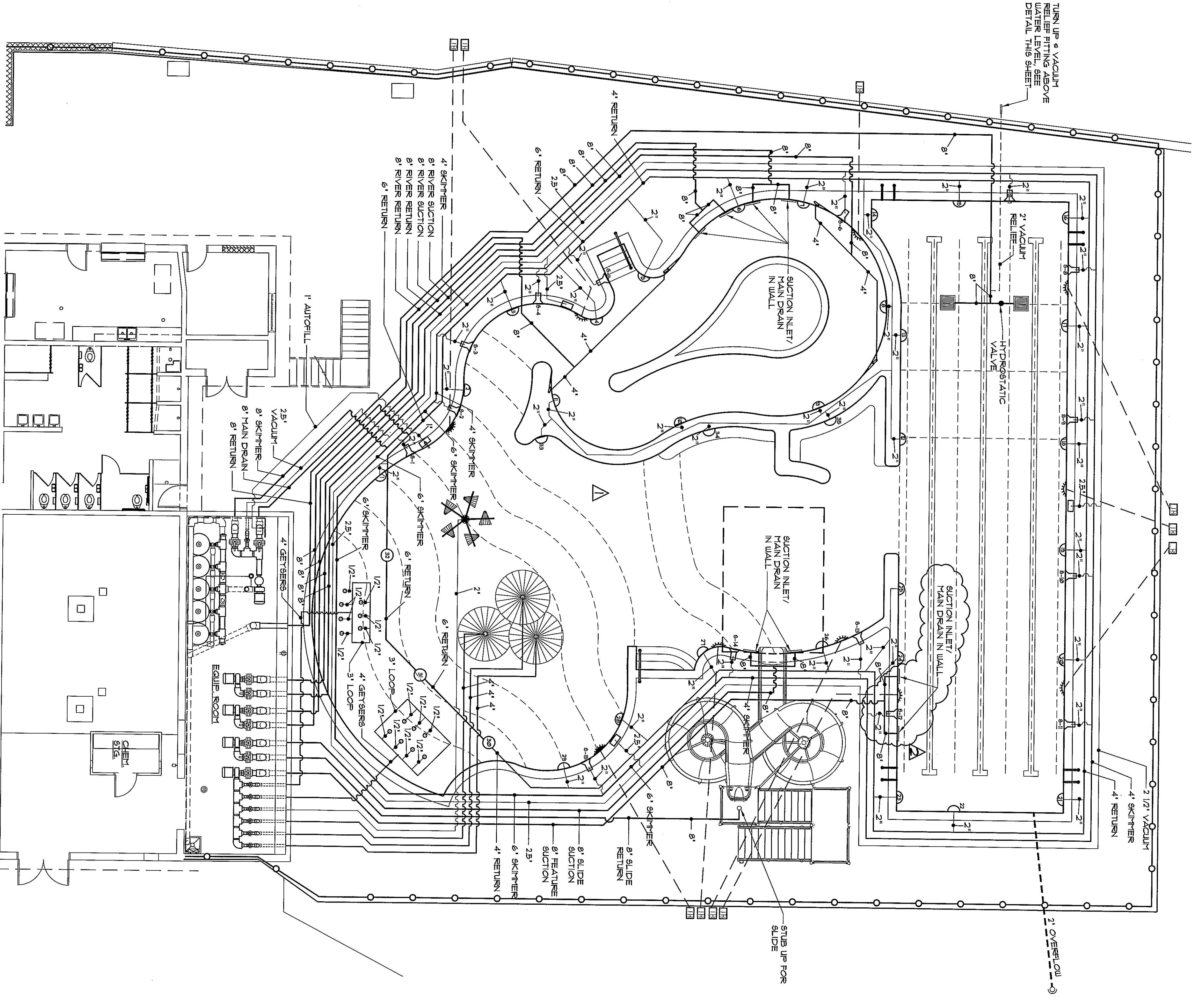
1 PIPING PLAN A-PL-4 1/8" = 1'-0"
